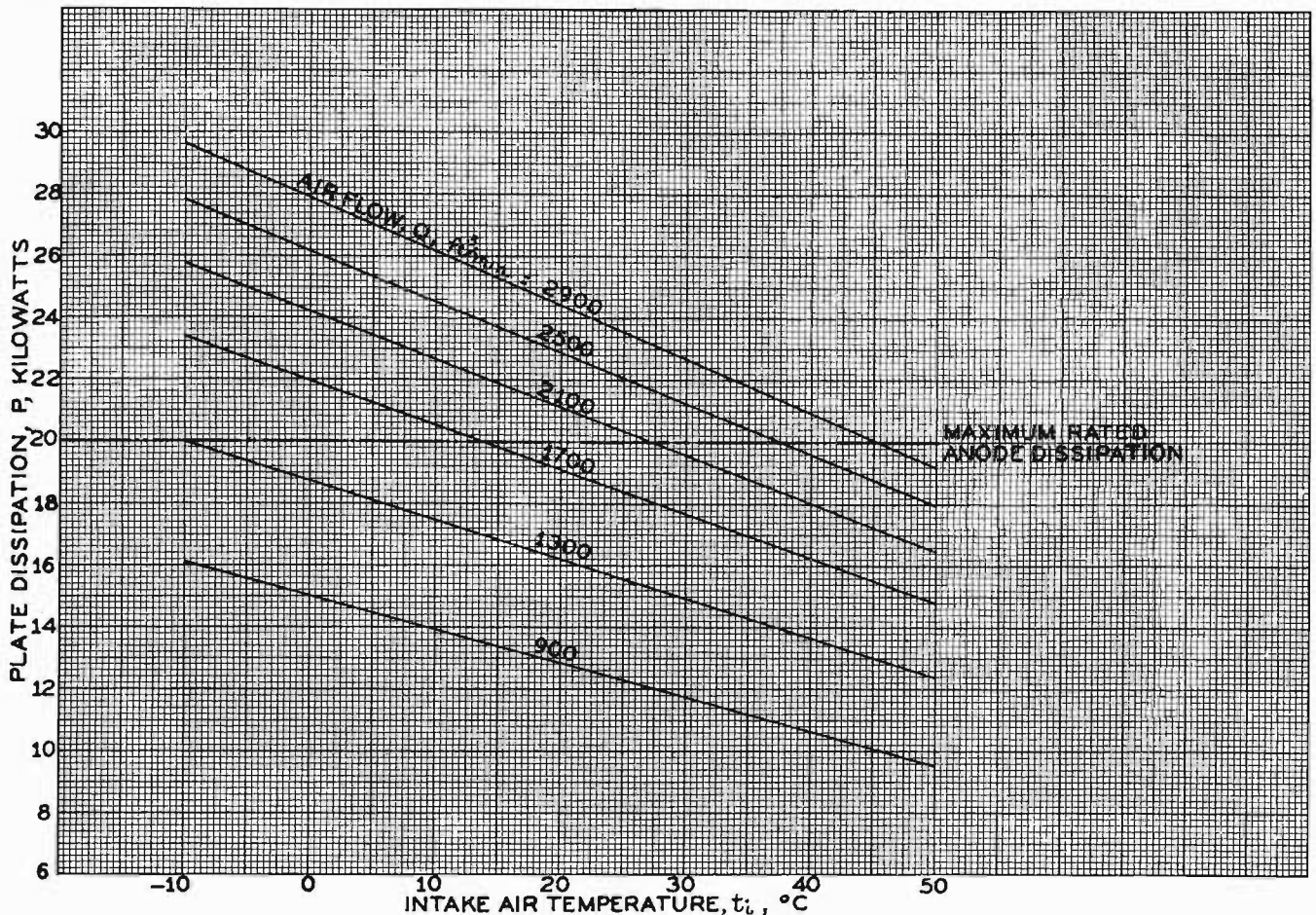
Fig. 1 Cooling Characteristics of Type F-124-R and F-125-R Forced-Air Cooled Tubes for Maximum Anode Temperature, T = 200^{\circ}\text{C}.
