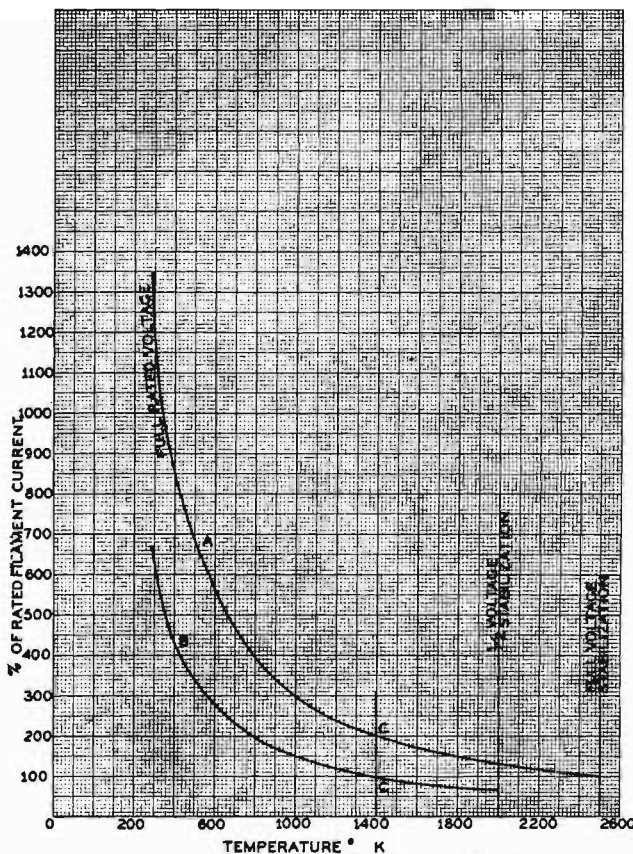
Fig. 1. Variation of Current with Temperature for Tungsten Filament for Half (curve B) and Full (curve A) Applied Voltage. Normal Operating Temperature = 2500° K.
